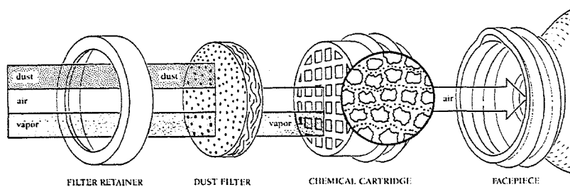
Figure 6-11. Pesticide cartridges consist of two stages. This diagram illustrates the mechanical dust filter which removes dust and droplet particles and the activated charcoal chemical cartridge which removes vapors.
