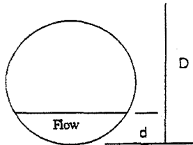
Figure 7-8. D is the diameter of the pipe and d is the depth of the flow. The wetted perimeter is that portion of the circumference submerged with water and the dry perimeter is the portion of the circumference above the water line.
