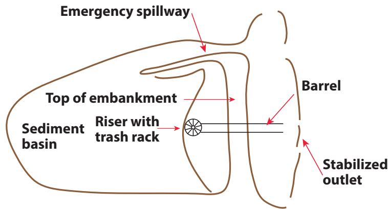
Figure 11. Sediment basin with spillway and release structure.
