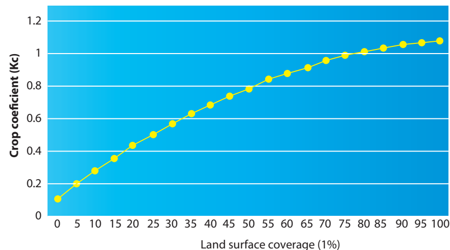
Figure 6. Relationship between crop coverage and crop coefficient.
